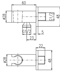
Mechanický STOP ventil Mechanical stop valve
